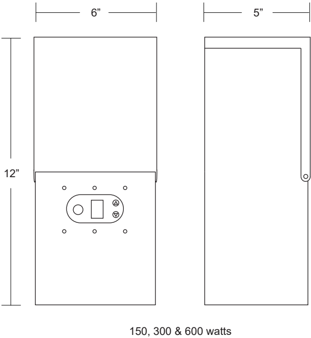
150, 300 & 600 watts
